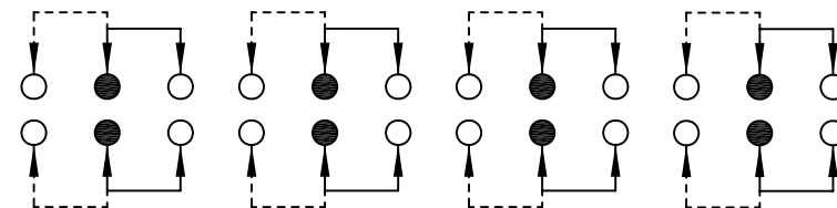
SCHEMATIC (NON-SHORTING)
